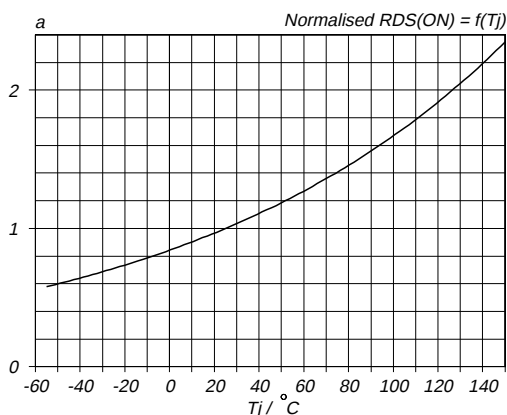
Fig.9. Normalised drain-source on-state resistance. a = R_{DS(ON)}/R_{DS(ON)25^\circ\text{C}} = f(T_J) ; I_D = 3.3 \text{ A} ; V_{GS} = 10 \text{ V}
