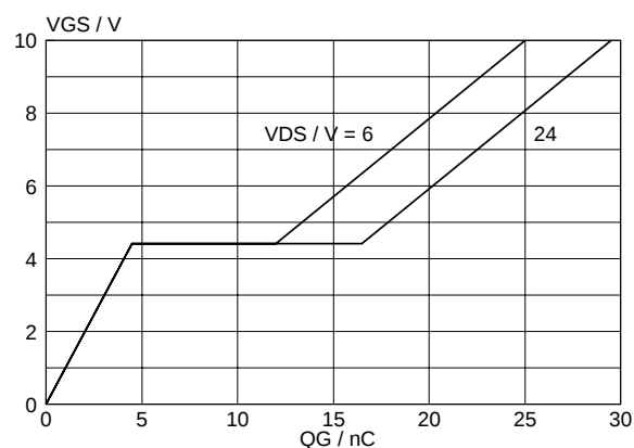
Fig.13. Typical turn-on gate-charge characteristics. V_{GS} = f(Q_G) ; conditions: I_D = 55 A; parameter V_{DS}
