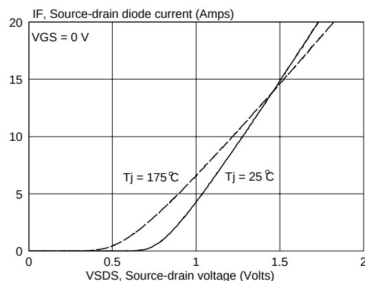
Fig.16. Source-Drain diode characteristic. I_F = f(V_{SDS}) ; parameter T_J
