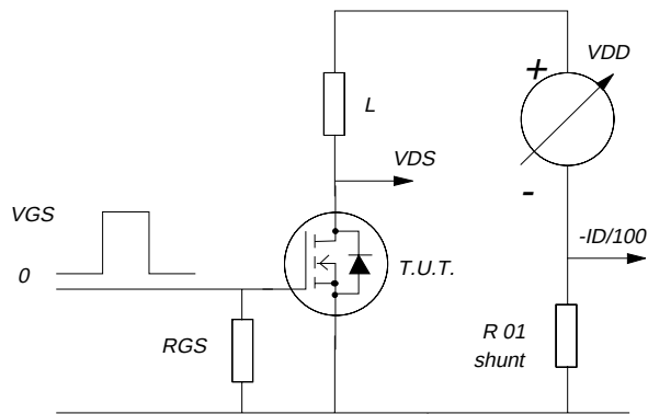
Fig.18. Unclamped inductive test circuit.
