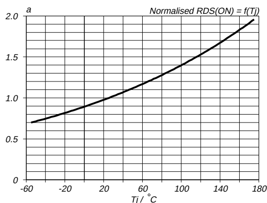
Fig. 9. Normalised drain-source on-state resistance. a = R_{DS(ON)}/R_{DS(ON)25^\circ\text{C}} = f(T_j) ; I_D = 10\text{ A} ; V_{GS} = 10\text{ V}
