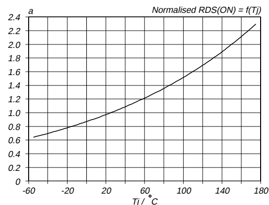
Fig.9. Normalised drain-source on-state resistance. a = R_{DS(ON)}/R_{DS(ON)25 \text{ °C}} = f(T_J) ; I_D = 5.6 \text{ A} ; V_{GS} = 5 \text{ V}
