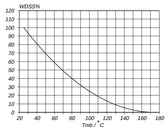
Fig.15. Normalised avalanche energy rating. W_{DSS}\% = f(T_{mb})
