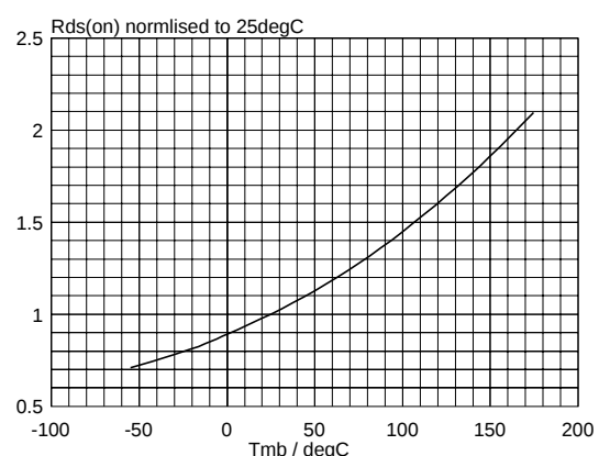
Fig.9. Normalised drain-source on-state resistance. a = R_{DS(ON)}/R_{DS(ON)25^\circ\text{C}} = f(T_j) ; I_D = 25\text{ A} ; V_{GS} = 5\text{ V}
