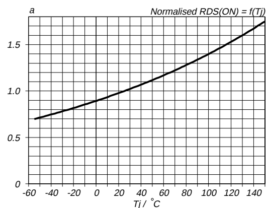
Fig.9. Normalised drain-source on-state resistance. a = R_{DS(ON)} / R_{DS(ON)25\text{ °C}} = f(T_j) ; I_D = 20 A; V_{GS} = 10 V
