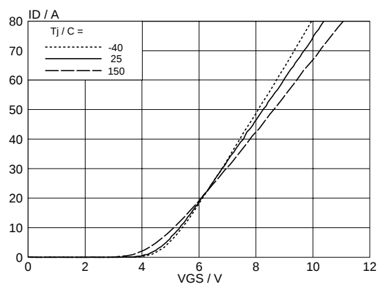
Fig.7. Typical transfer characteristics. I_D = f(V_{GS}) ; conditions: V_{DS} = 15 V; parameter T_j
