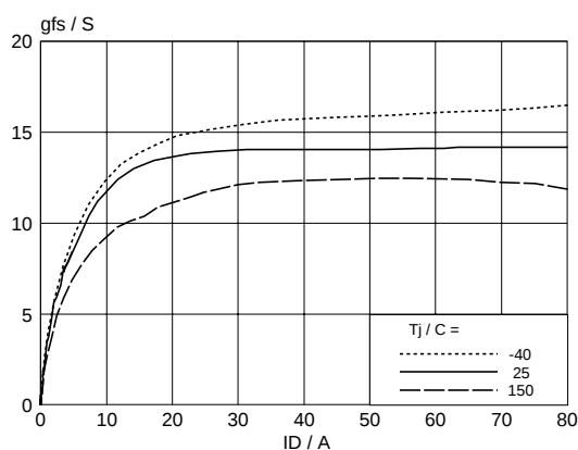
Fig.8. Typical transconductance, T_j = 25 °C. g_{fs} = f(I_D) ; conditions: V_{DS} = 15 V
