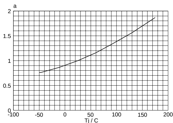
Fig. 9. Normalised drain-source on-state resistance. a = R_{DS(ON)}/R_{DS(ON)25\text{ °C}} = f(T_j) ; I_D = 25\text{ A} ; V_{GS} = 5\text{ V}
