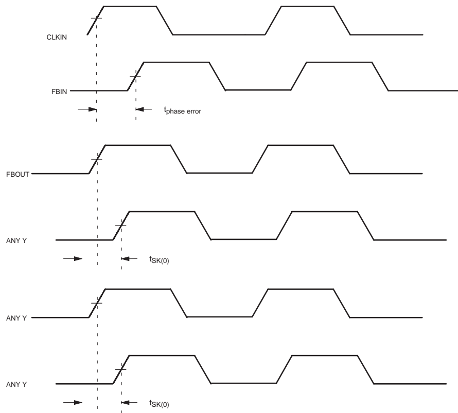
Figure 2. Phase Error and Skew Calculations
