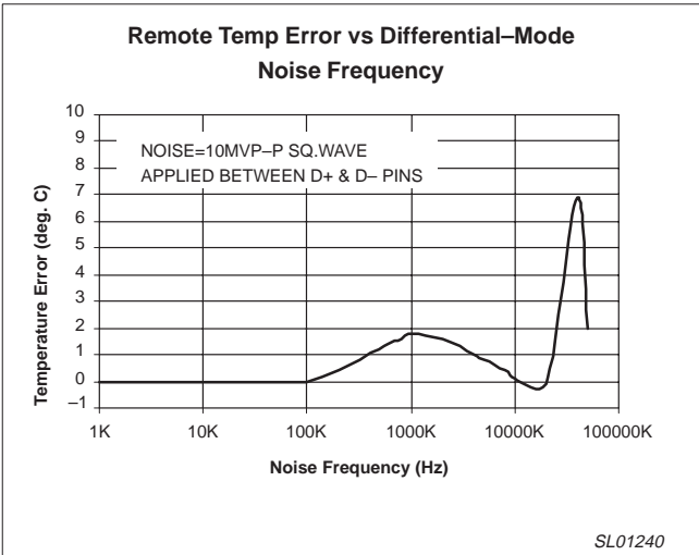
Figure 7. Temp error vs Different Mode Noise Frequency
