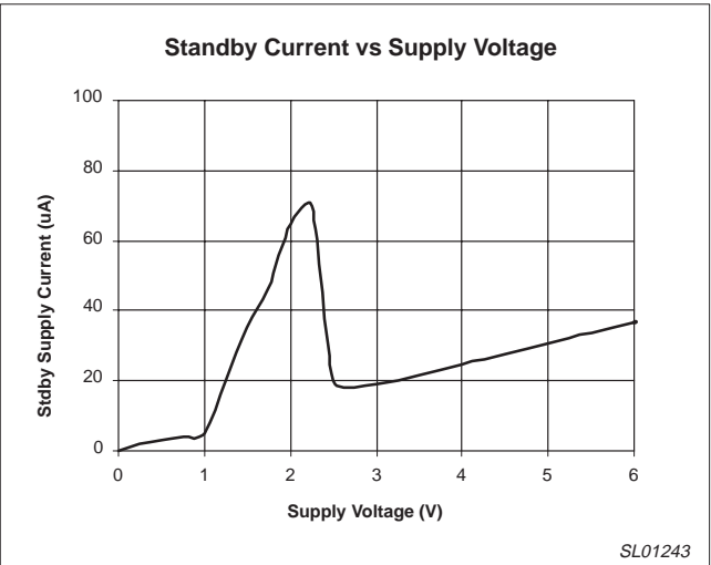
Figure 3. Standby Current vs Supply Voltage
