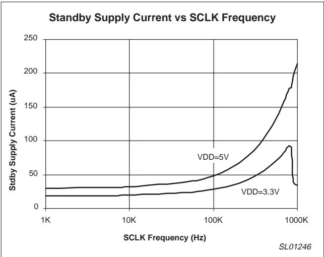
Figure 5. Standby Current vs SCLK Frequency
