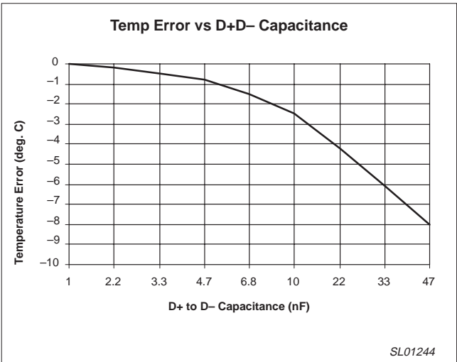
Figure 2. Temp Error vs D+D- Capacitance
