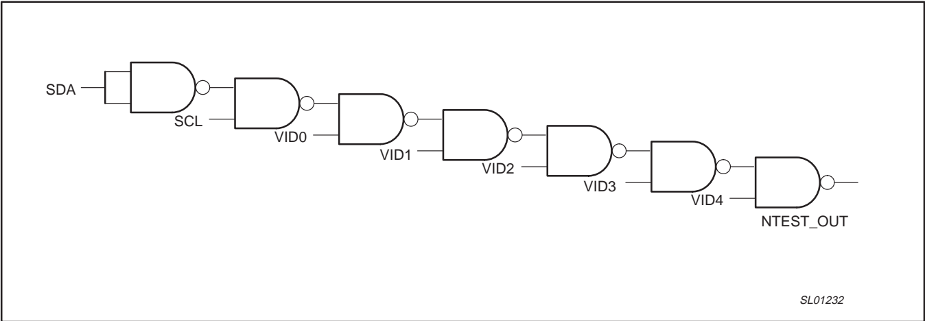
Figure 1. NAND-tree circuitry
