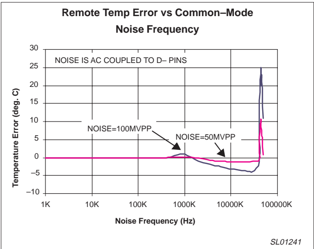
Figure 6. Temp Error vs Common Mode Noise
