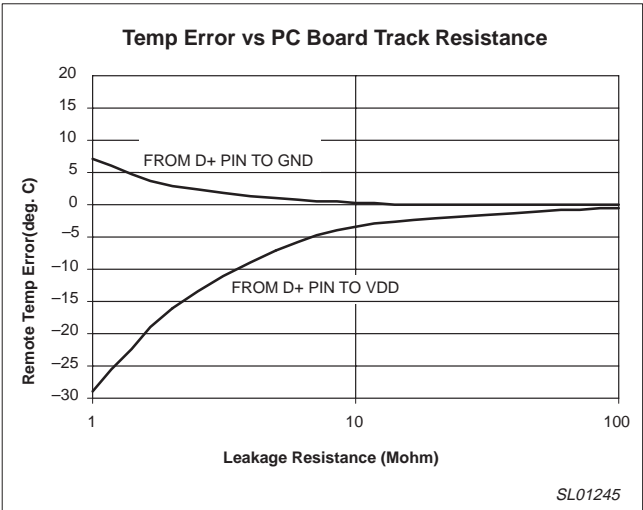
Figure 1. Temp Error vs PC Board Track Resistance
