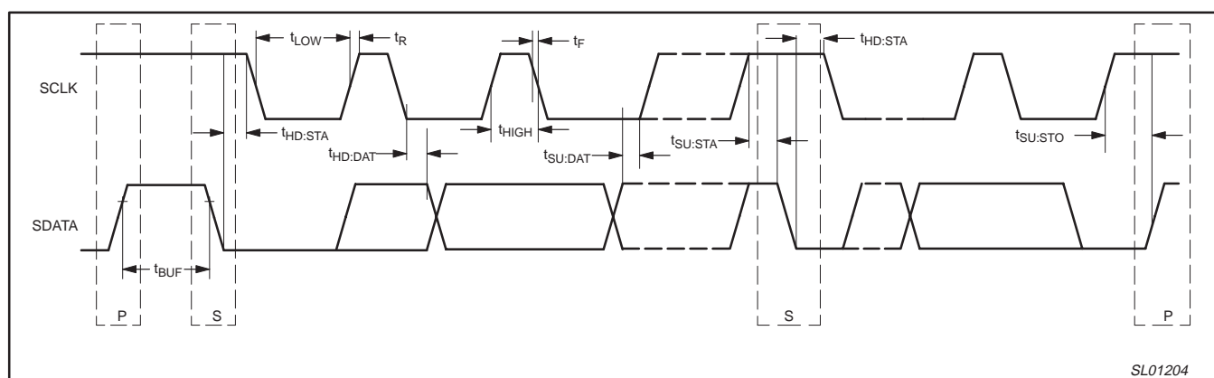
Figure 3. Timing Measurements
