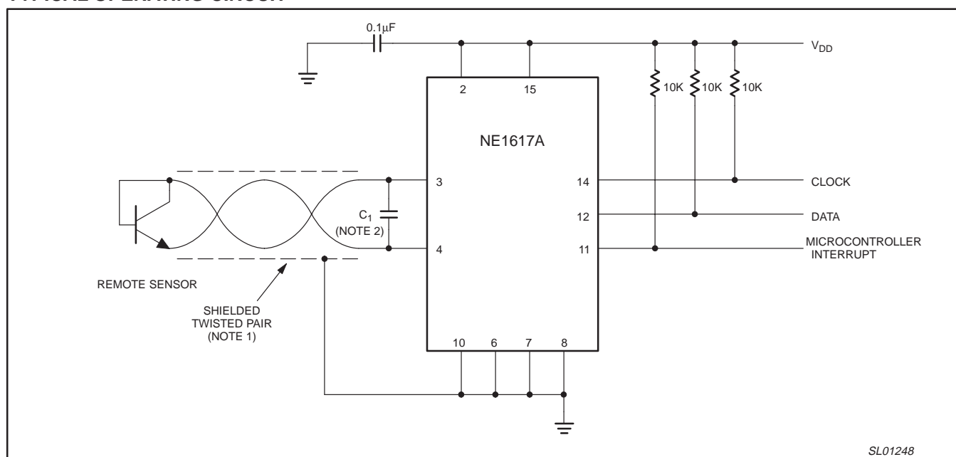
Figure 2. Typical operating circuit
