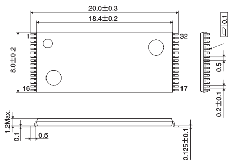
TSOP32 (pre liminary)
