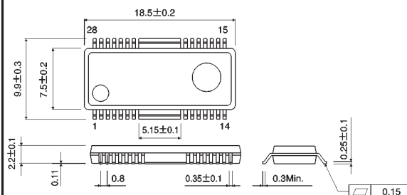
HSOP28/HSOP-M28
