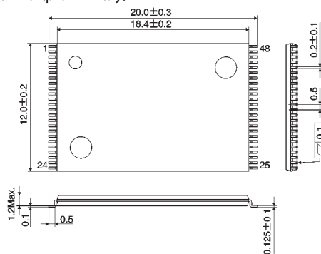
TSOP48 (pre liminary)
