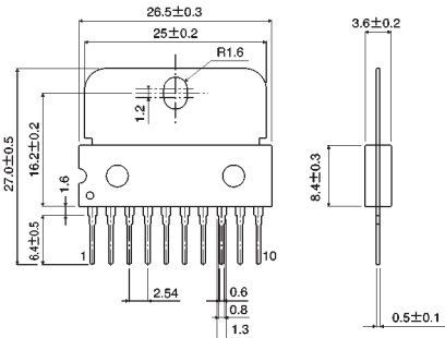
HSIP10
