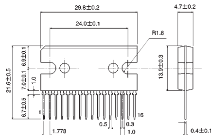
SIP-M16
