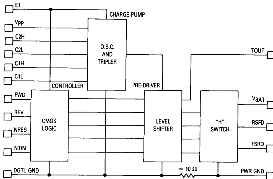
Figure 1. Block Diagram
