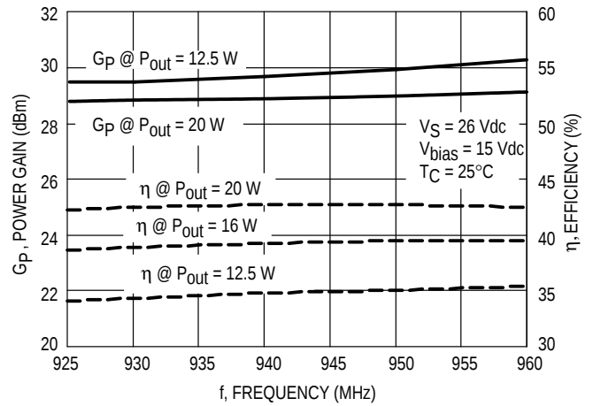
Figure 2. Power Gain and Efficiency versus Frequency
