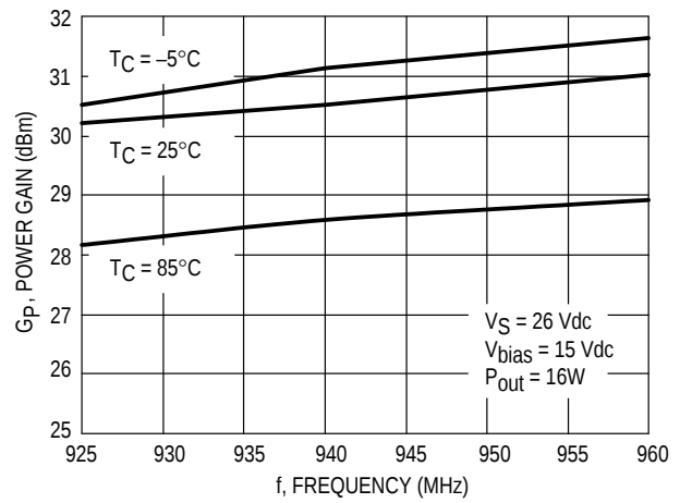
Figure 4. Power Gain versus Frequency
