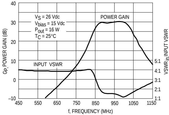
Figure 1. Power Gain and Input VSWR versus Frequency
