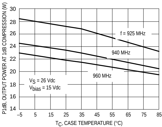
Figure 5. Output Power at 1 dB Compression versus Temperature
