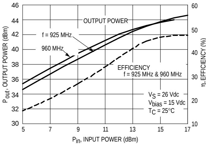
Figure 3. Output Power and Efficiency versus Input Power
