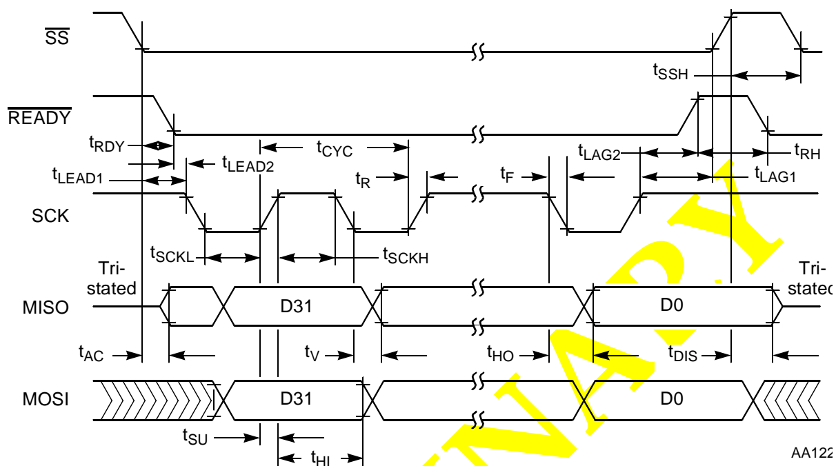
Figure 2-3 SPI Timing
