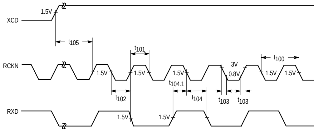
Figure 16. Receive Timing (Fujitsu Start of Frame)
