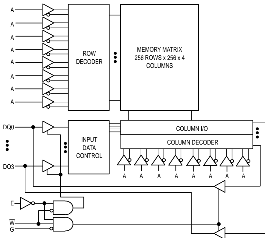
BLOCK DIAGRAM
