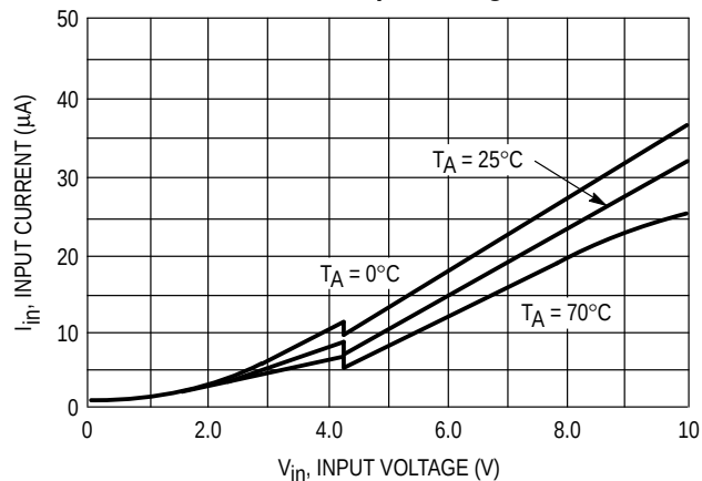
Figure 8. MC3X164-5 Input Current versus Input Voltage
