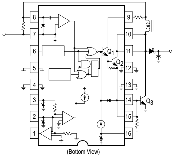
Figure 23A. External NPN Switch
