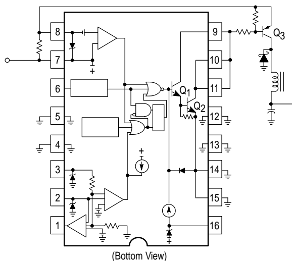
Figure 21B. External PNP Saturated Switch
