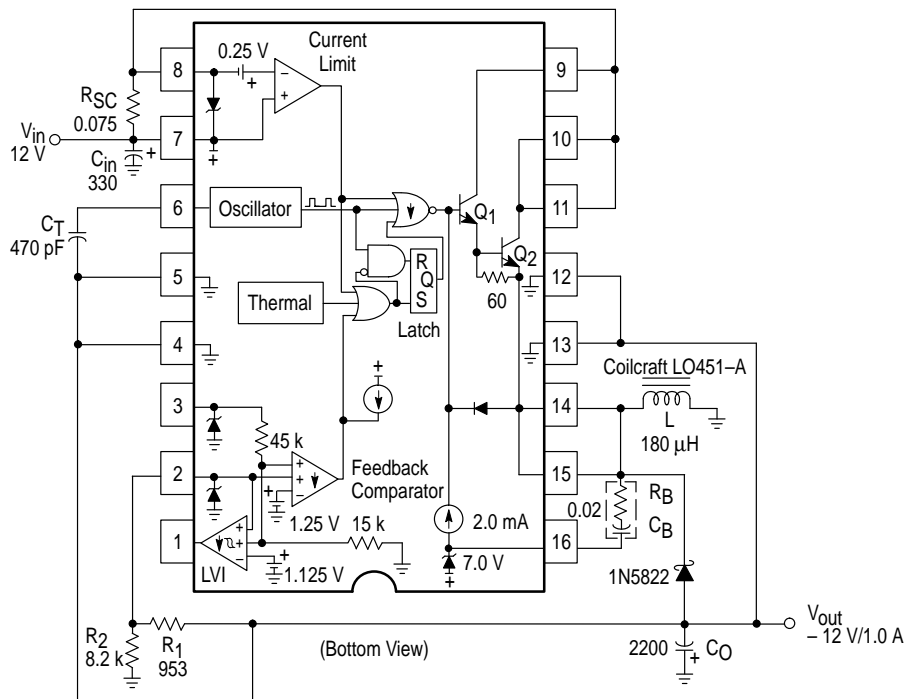
Figure 24. Voltage-Inverting Converter
