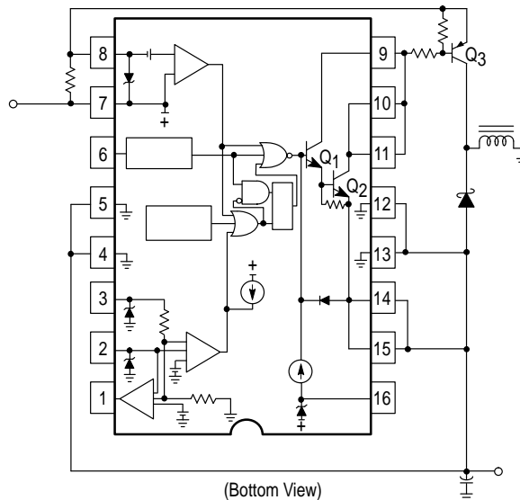
Figure 25B. External PNP Saturated Switch
