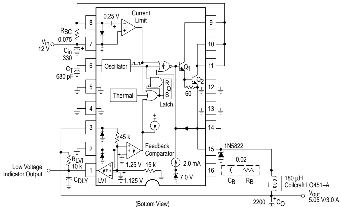
Figure 20. Step-Down Converter
