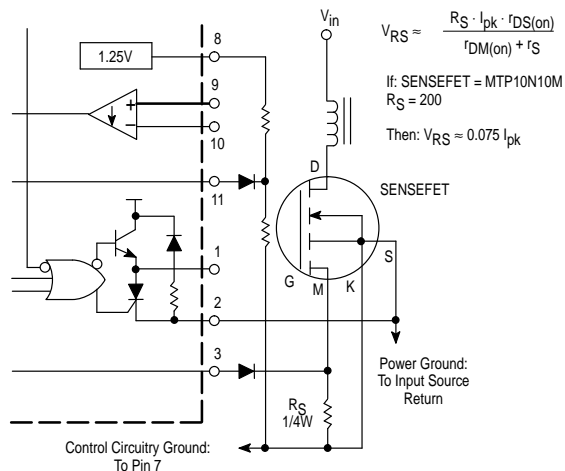
Figure 24. Current Sensing Power MOSFET
