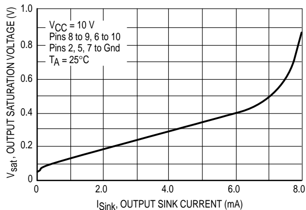
Figure 8. Error Amp Output Saturation versus Sink Current
