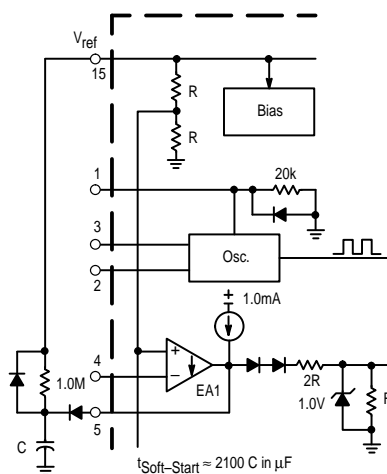
Figure 20. Soft-Start Circuit
