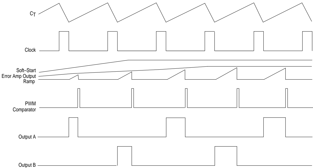
Figure 19. Current Limit Operating Waveforms
