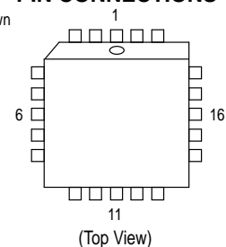
FN SUFFIX PLASTIC PACKAGE CASE 775 (PLCC)
