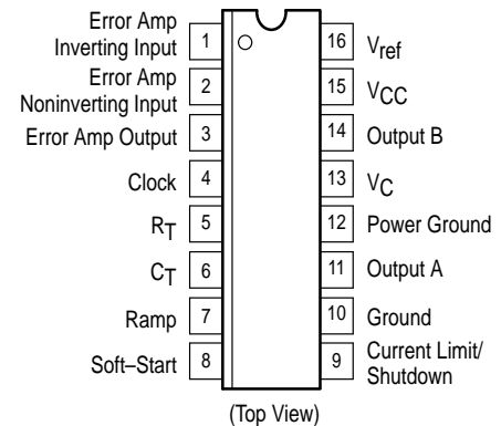
DW SUFFIX PLASTIC PACKAGE CASE 751G (SO-16L)
