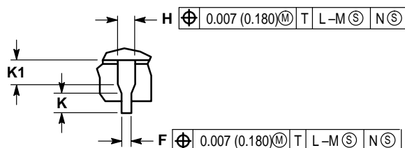
VIEW S
