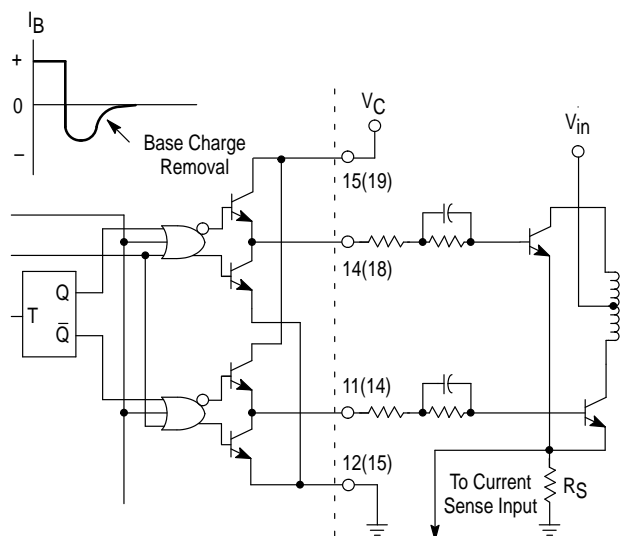
Figure 32. Bipolar Transistor Drive
