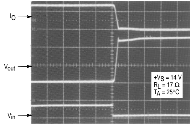
Figure 12. Turn-Off Waveform
