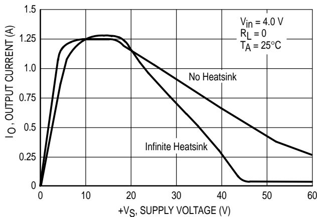
Figure 13. Output Current versus Supply Voltage
