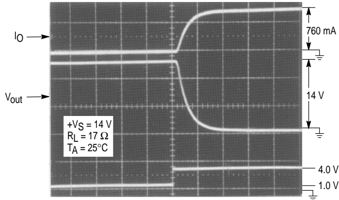
Figure 11. Turn-On Waveform
