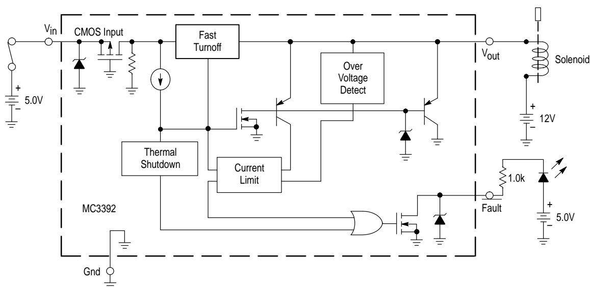
Figure 15. Solenoid Driver
