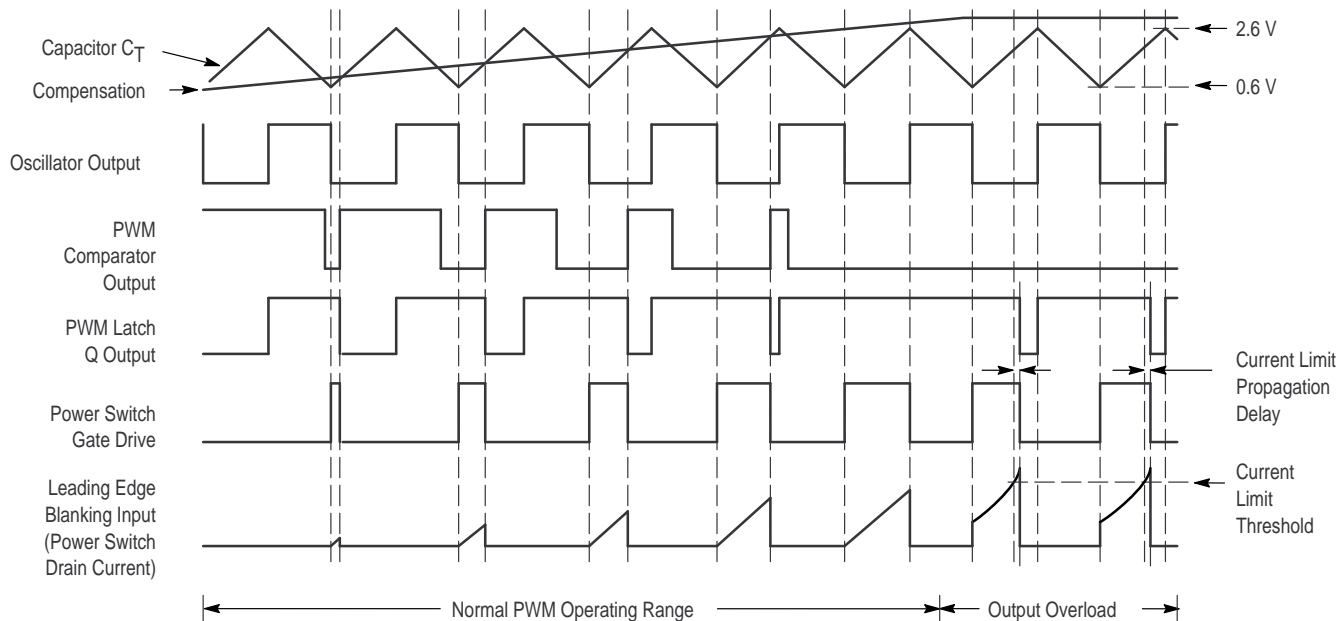
Figure 18. Timing Diagram
