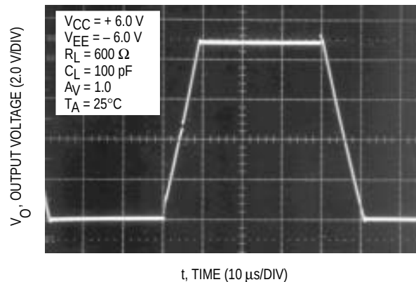
Figure 28. Large Signal Transient Response
