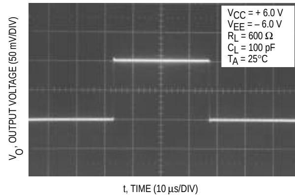
Figure 27. Small Signal Transient Response
