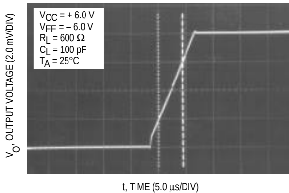
Figure 26. Noninverting Amplifier Slew Rate
