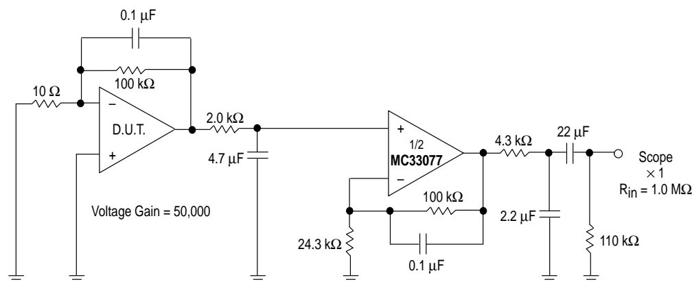
Figure 36. Voltage Noise Test Circuit (0.1 Hz to 10 Hzp-p)
