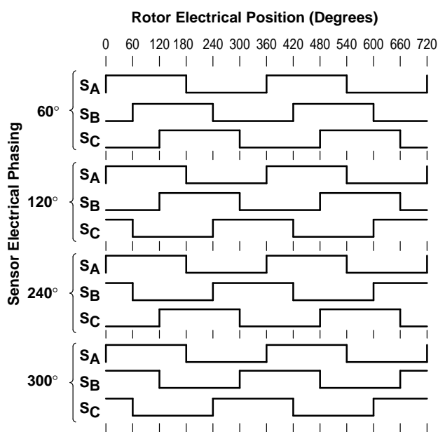
Figure 41. Sensor Phasing Table
