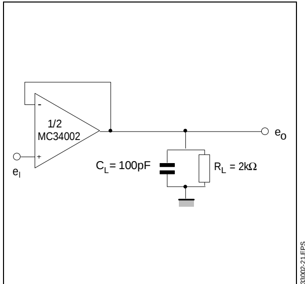
Figure 1 : Voltage Follower
