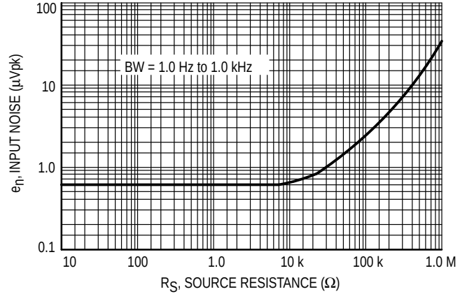
Figure 2. RMS Noise versus Source Resistance
