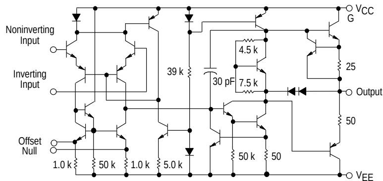
Equivalent Circuit Schematic (1/4 of Circuit Shown)
