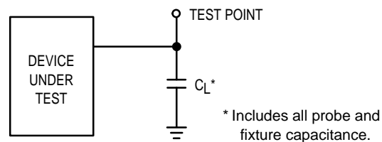
Figure 12. Test Circuit
