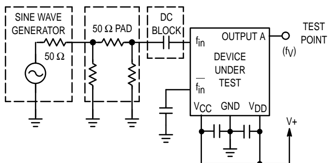
Figure 7. Test Circuit
