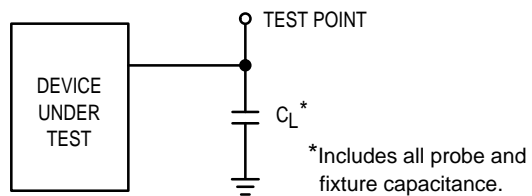
Figure 12. Test Circuit
