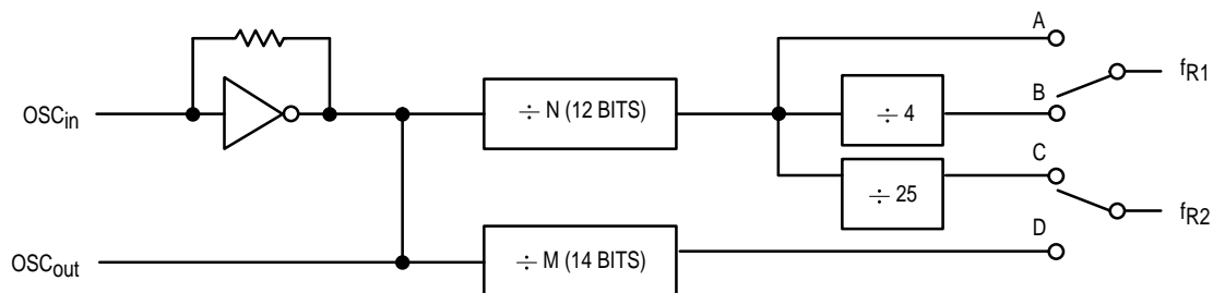
Reference Frequency vs Crystal Frequency
