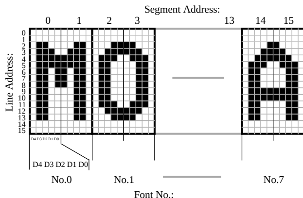
Figure 12. Memory Map of Programmable RAM Fonts
