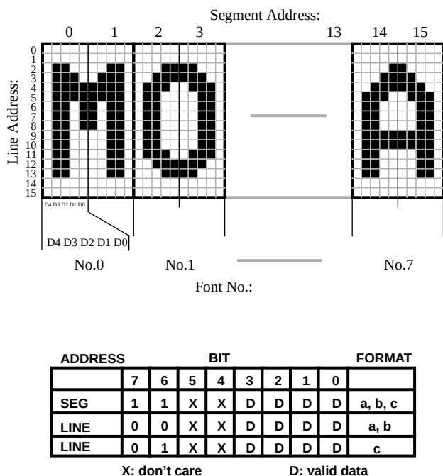
Figure 9. Address Bit Patterns for RAM Fonts
