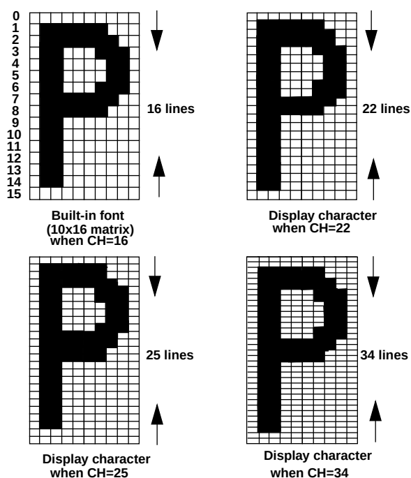
Figure 13. Variable Character Height
