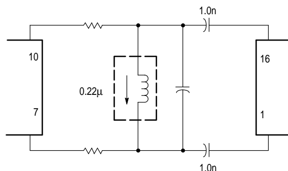
Network Topology
