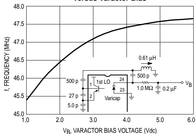
Figure 5. Oscillator Frequency versus Varactor Bias
