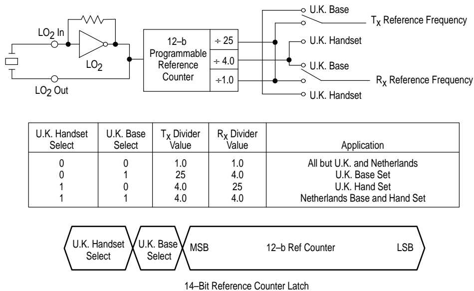
Figure 13. Reference Counter Register Programming Mode
