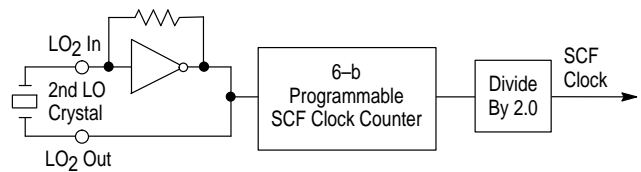
Figure 27. SCF Clock Circuit
