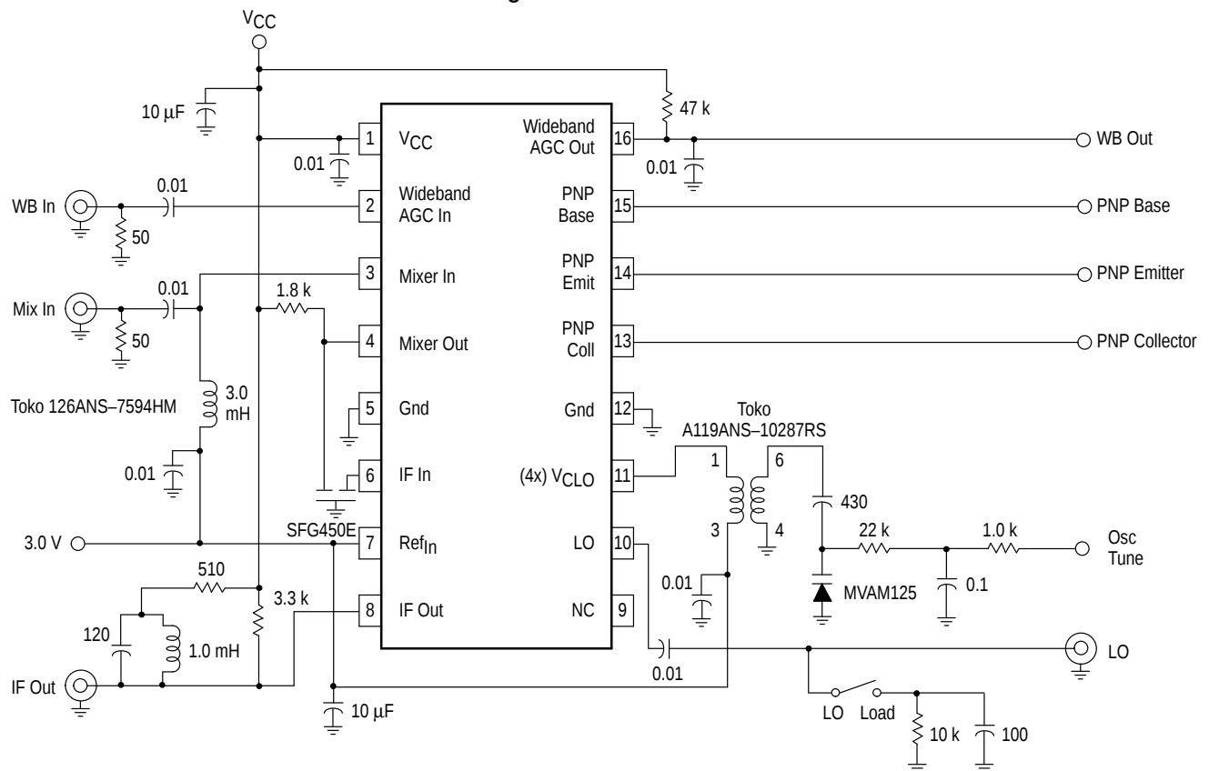
Figure 1. Test Circuit
