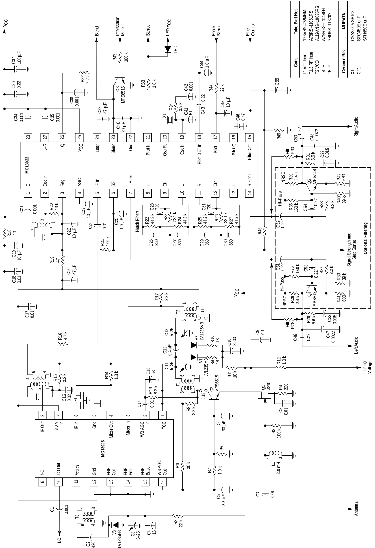
Figure 2. Cascode RF ETR Application (NPSC – Notch Filters – Optional Pilot High Pass)
