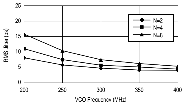
Figure 5. RMS PLL Jitter versus VCO Frequency
