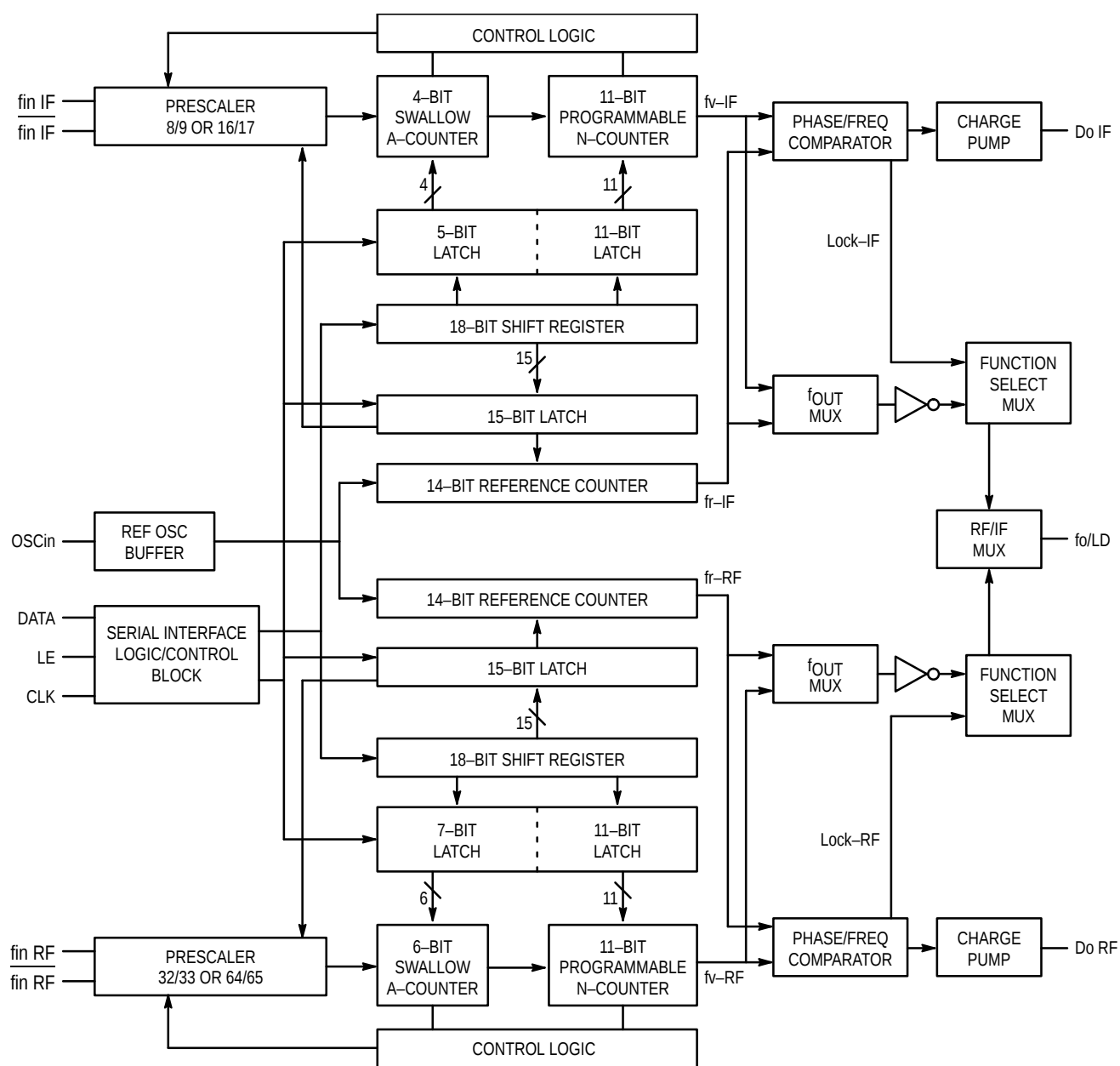
Figure 1. MC12310 Functional Block Diagram
