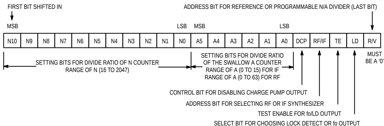
DIVIDE RATIO OF PROGRAMMABLE N-COUNTER
