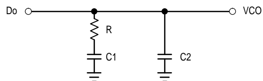
Figure 7. Typical Loop Filter
