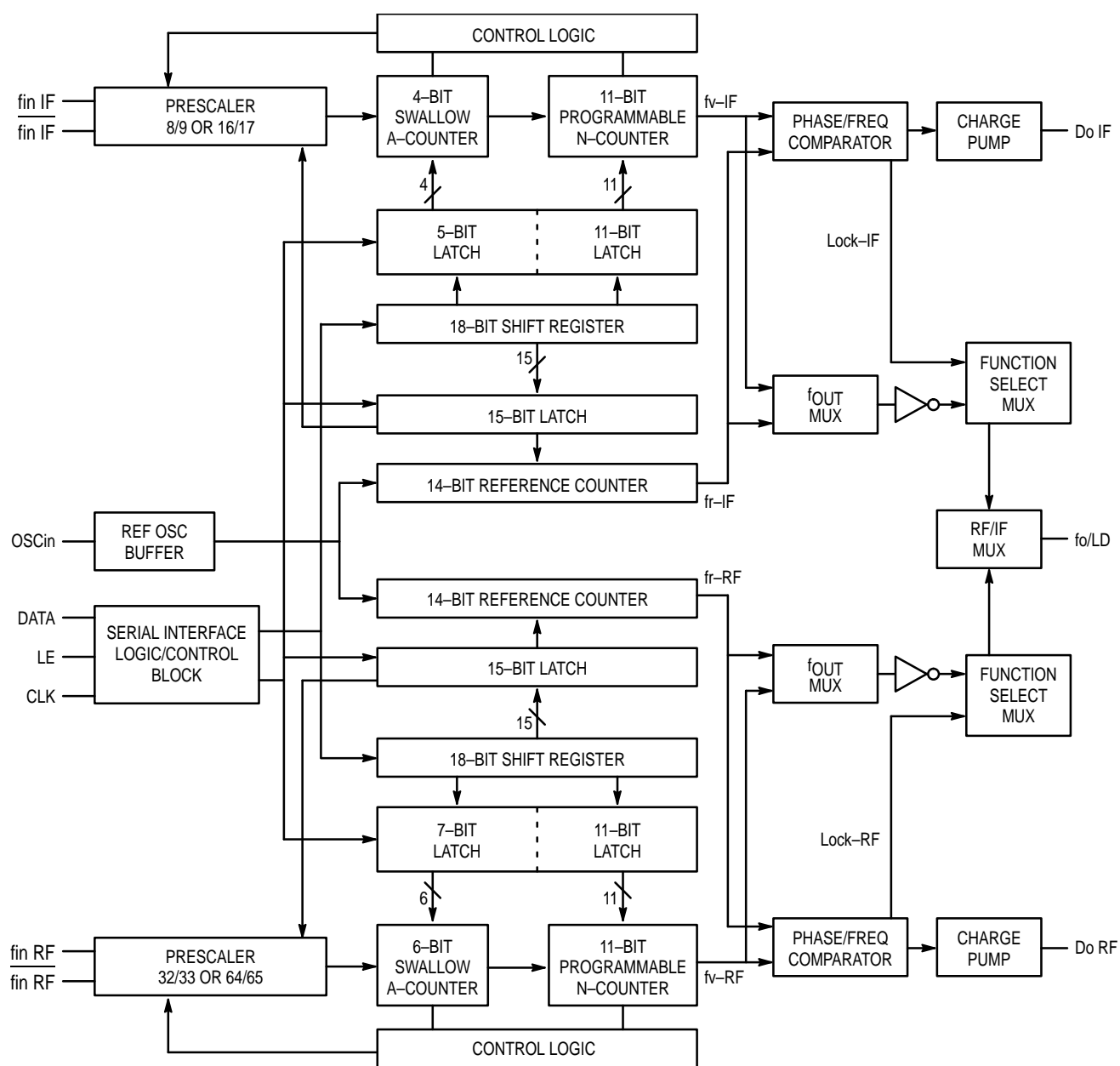
Figure 1. MC12302 Functional Block Diagram
