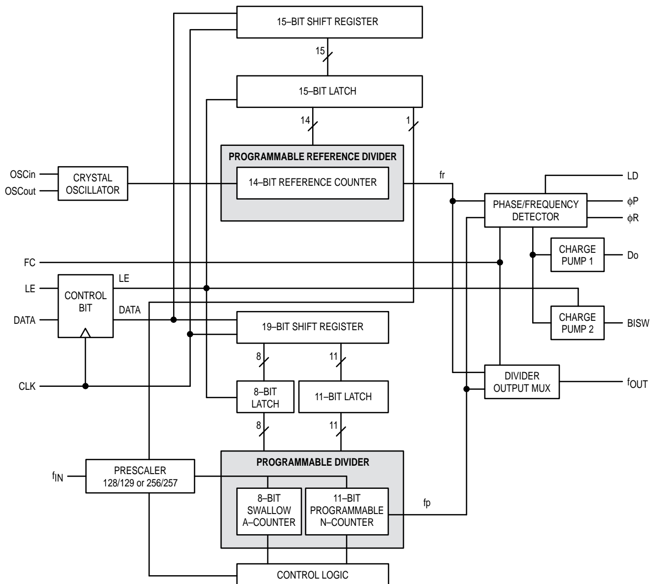
Figure 1. MC12207 Block Diagram
