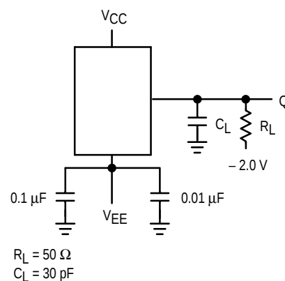
Figure 2. AC Test Circuit
