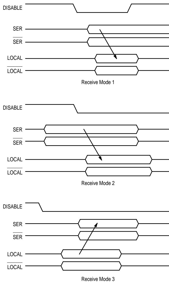
Figure 4. Functional Timings
