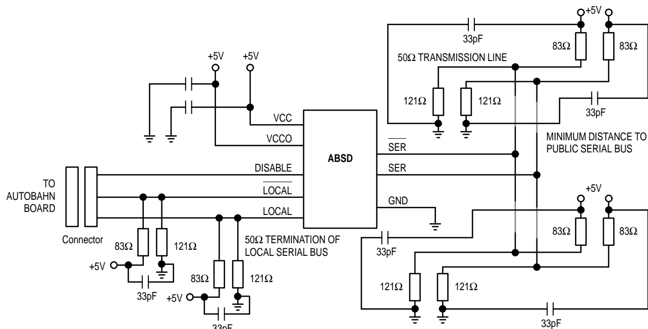
Figure 5. ABSD Interface Design
