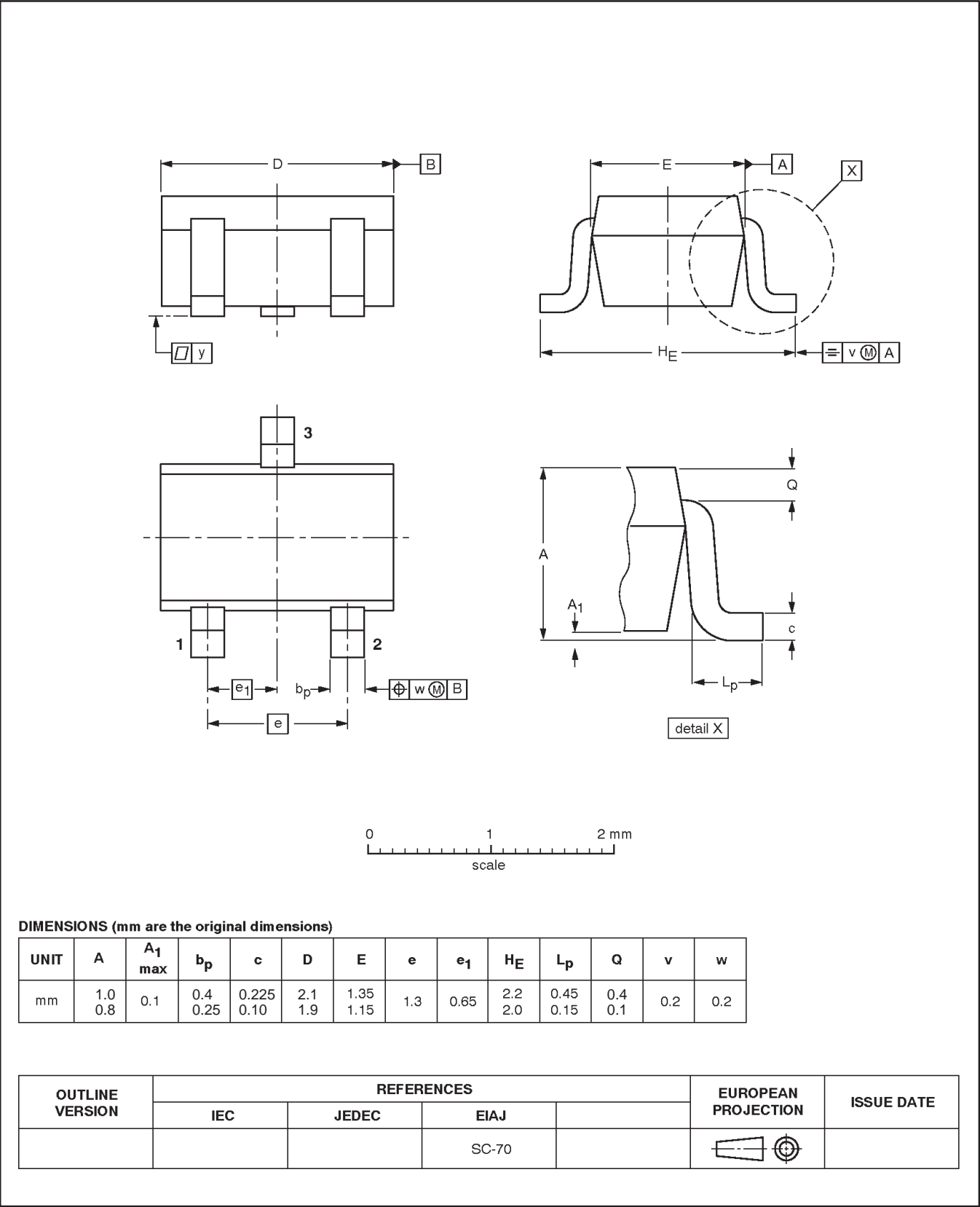
SC70-3: plastic small outline package; 3 leads; body width 1.15 mm
