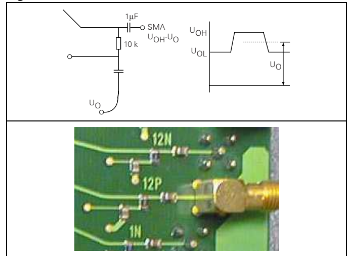
Figure 13 Pad locations for LVDS level measurements
