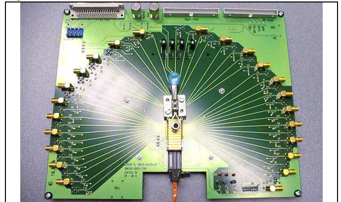
Figure 3 Test board PAROLI receiver AC/DC
