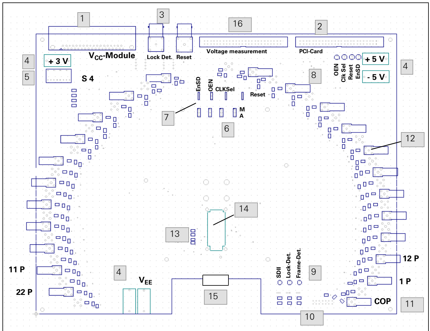
Figure 18 PAROLI receiver test board layout
