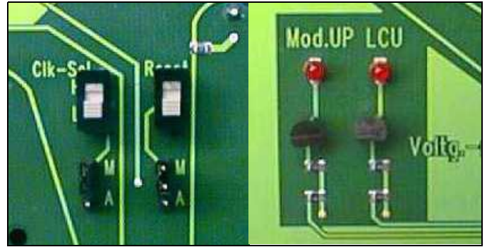
Figure 2 Switch, jumpers and LEDs on the Tx test board
