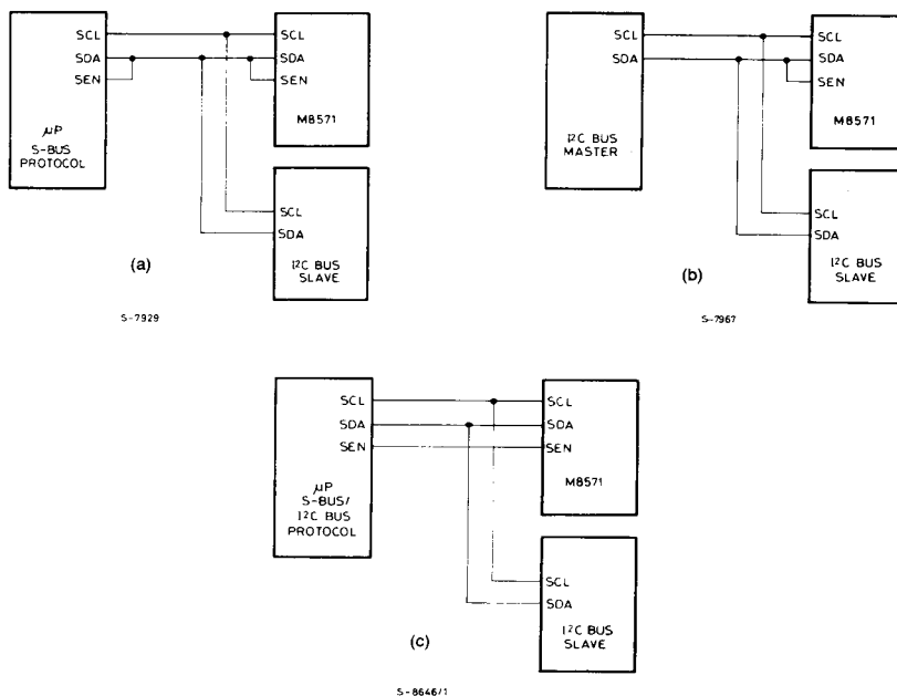
Fig. 5 - SYSTEM WITH "MIXED" S-BUS/I 2 C BUS PERIPHERAL
