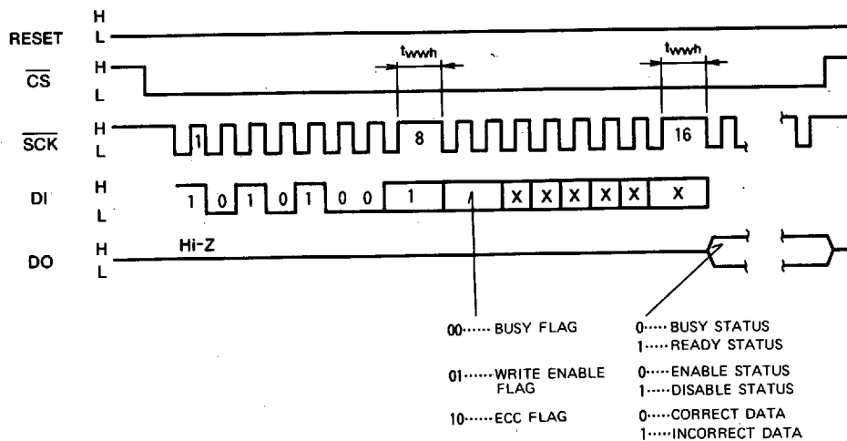
Fig. 3 Sequence at status output mode
