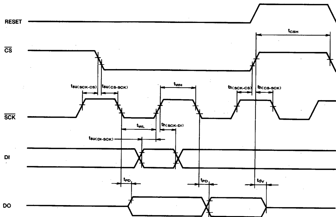
Fig. 1 Synchronizing timing
