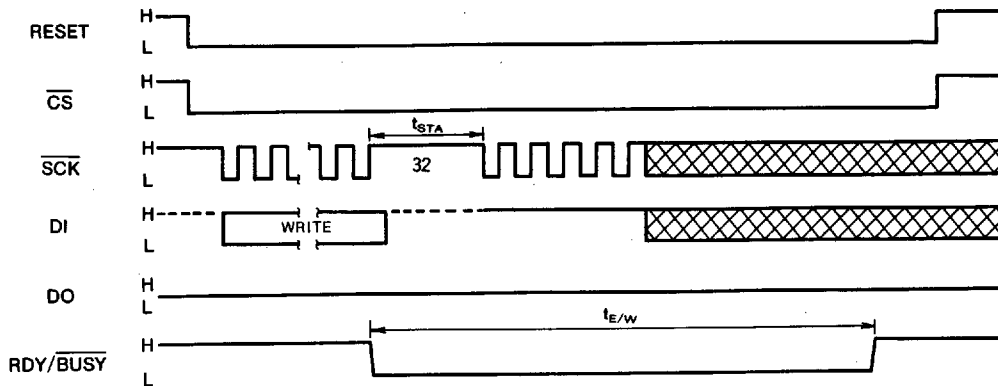
Fig. 10 Sequence of write operation
