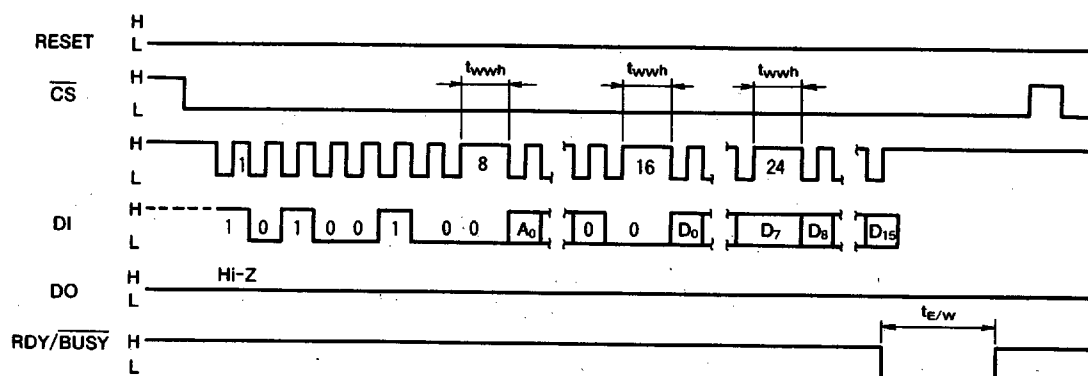
Fig. 5 Sequence at write mode
