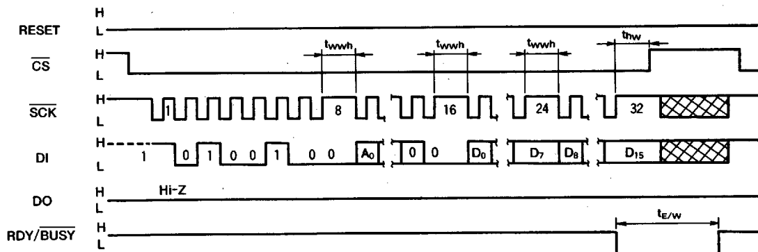
Fig. 6 Sequence at write mode
