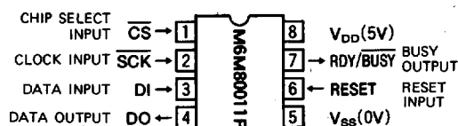
Outline 8P4
