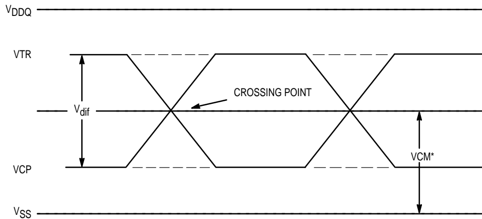
Figure 3. Differential Inputs/ Common Mode Input Voltage
