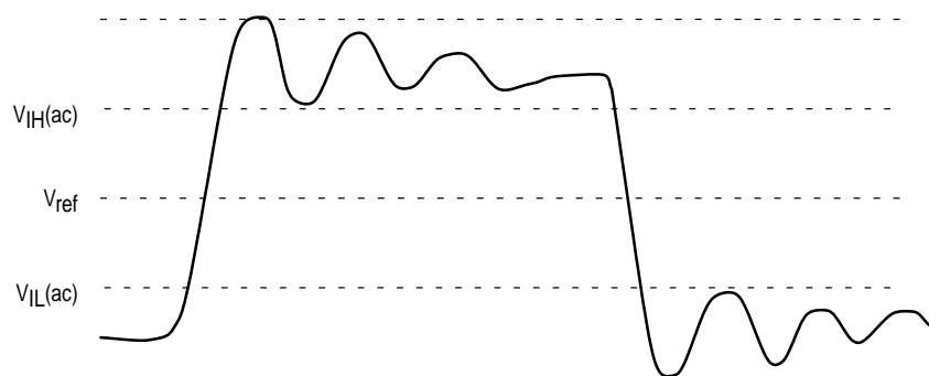
Figure 3. Differential Inputs/ Common Mode Input Voltage
