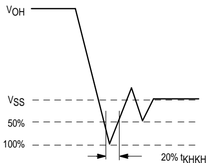
Figure 1. Undershoot Voltage
